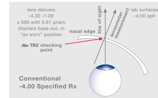
Lab surfaces to the specified prescription, but delivers a certain amount of prism and prescription errors in the "as worn" position due to the wrap angle of the frame.
